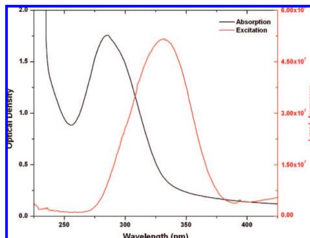
Figure 1. Absorption and excitation (614 nm) spectra.
