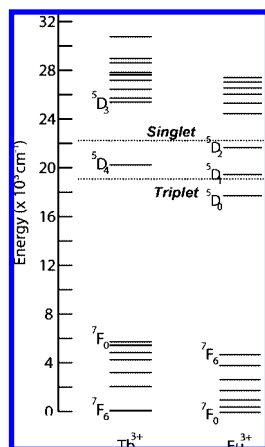
Figure 3. Position of the ligand singlet and triplet energy states and corresponding \text{Eu}^{3+} and \text{Tb}^{3+} energy states.
